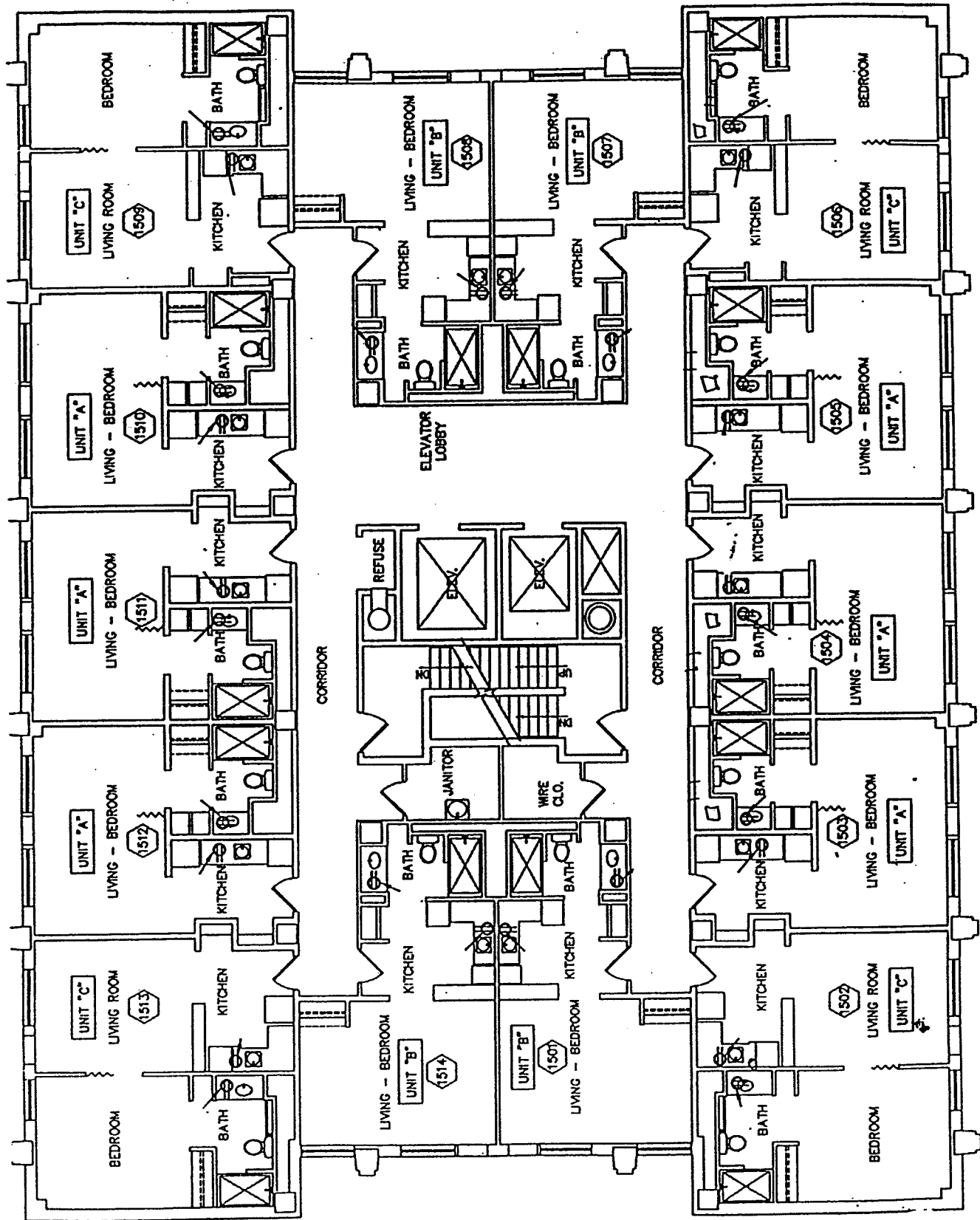
PAQUIN FLOOR PLANS 2 THRU 15
